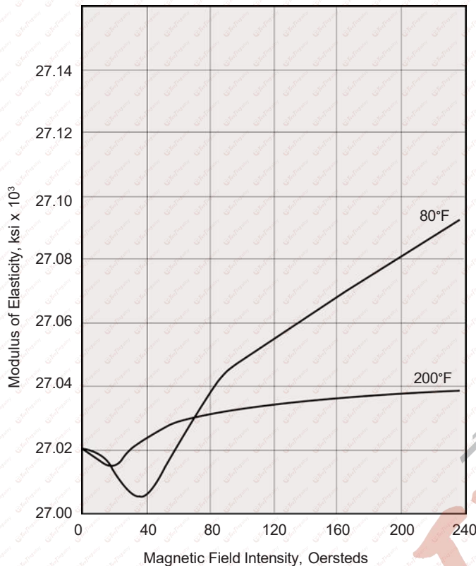
Figure 14. Effect of magnetic field intensity on modulus of elasticity at two temperatures. Material cold rolled 40% and heat treated 1000°F/5 hours prior to testing.
